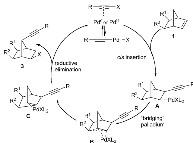
Scheme 9. Proposed mechanism for the bromoalkynylation reaction.
